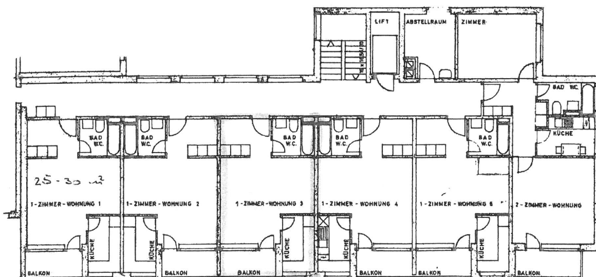
GRUNDRISS STOCK
